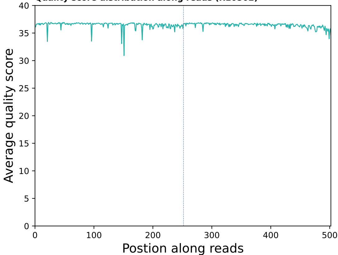
Quality score distribution along reads (R10502)
